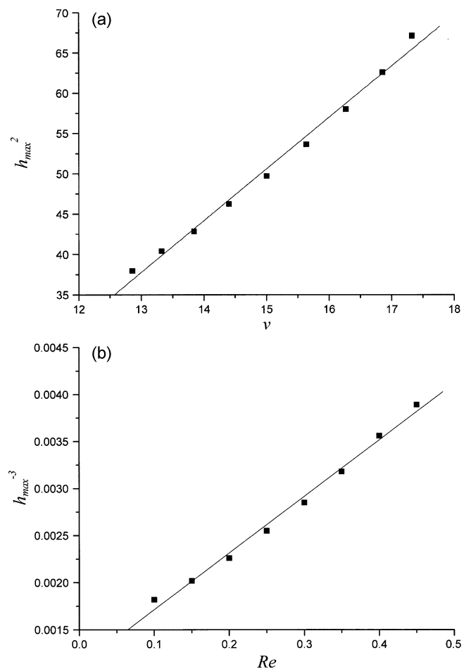
Fig. 8. (a) v versus h_{max}^2 for B=5 , 1/Ca=3,000 , K=10 and H=10 . (b) Re versus h_{max}^{-3} for B=5 , 1/Ca=3,000 , K=10 and H=10 .
